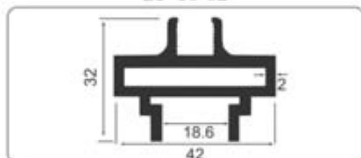
Horizontal Profile For 10mm Glass (10mmx42mm) Finish : Black Matt Available in : 10ft and 16ft
