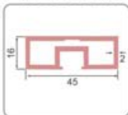
SP-16-11 BRG
