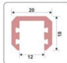
Edge Profile for 12mm Glass (20mm) Finish : Brush Rose Gold
