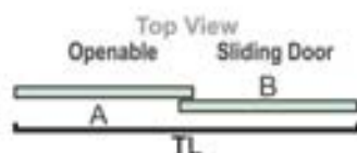
SP-PTD 1+1-02 (W 1800mmxH 2700mm) Sliding and Opening of 2 Door
