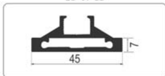
Vertical Profile for 10mm Glass Finish : Black Matt
