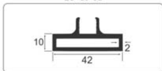
Vertical Profile For 10mm Glass (10mmx42mm) Finish : Black Matt Available in : 10ft and 16ft
