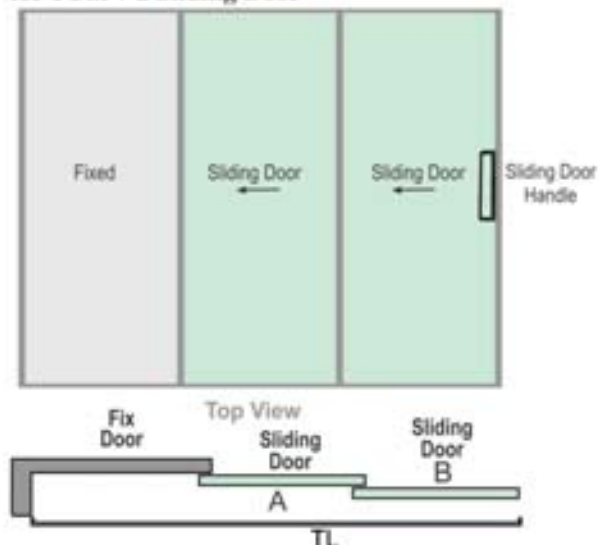
Telescopic Sliding Door Hardware for 1 Fix + 2 Sliding Door
