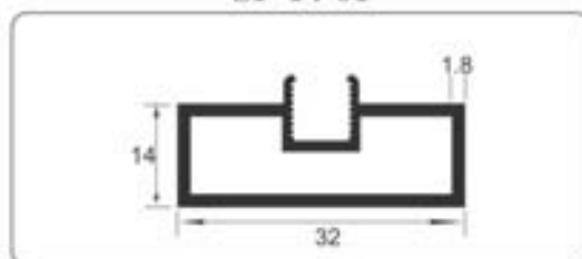
Vertical Profile For 8mm Glass (10mmx42mm) Finish : Black Matt Available in : 10ft and 16ft
