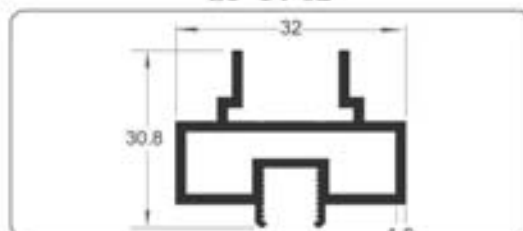
Horizontal Profile For 8mm Glass (10mmx42mm) Finish : Black Matt Available in : 10ft and 16ft
