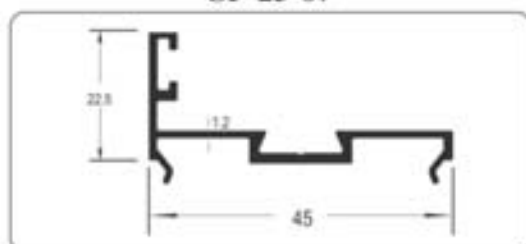
Slim Profile (25mmx45mm) Finish : Black Matt Available in : 10, 16ft.
