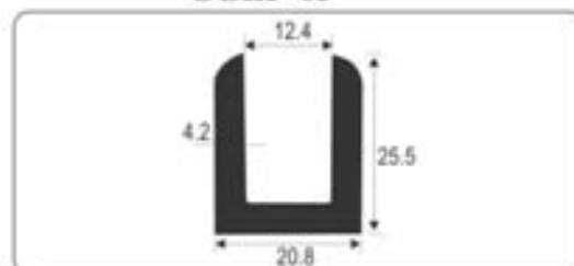
Profile for 12mm Glass Partition (25mm) Finish : Black Matt
