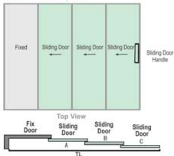
Telescopic Sliding Door Hardware for 1 Fix + 3 Sliding Door
