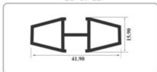
Center Profile for 10mm Glass Finish : Black Matt
