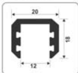
Edge Profile for 12mm Glass (20mm) Finish : Black Matt
