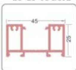
Slim Profile Finish : Brush Rose Gold
