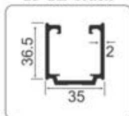
Sliding Top Track Finish : Black Matt Available in : 2, 3, 4, 5mtr
