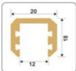
Edge Profile for 12mm Glass (20mm) Finish : Metallic Gold
