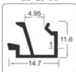
Slim Profile Cover Bidding (25mmx45mm) Finish : Black Matt Available in : 10, 16ft.
