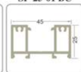
Slim Profile Finish : Brush Champagne
