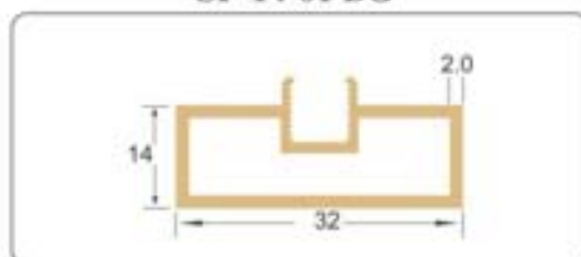
Vertical Profile For 8mm Glass (14mmx32mm) Finish : Brush Gold Available in : 10ft and 16ft
