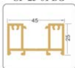
Slim Profile Finish : Brush Gold
