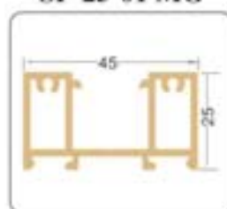
Slim Profile Finish : Metallic Gold
