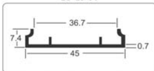
Slim Profile Cover (25mmx45mm) Finish : Black Matt Available in : 10, 16ft.
