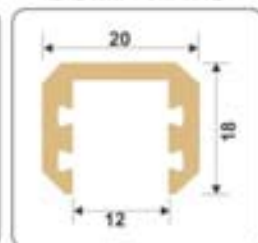
Edge Profile for 12mm Glass (20mm) Finish : Brush Gold
