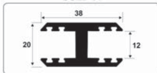
Profile for 12mm Glass (38mm) Finish : Black Matt
