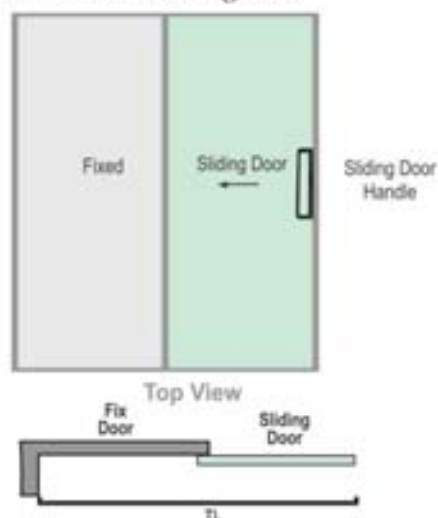
Telescopic Sliding Door Hardware for 1 Fix + 1 Sliding Door
