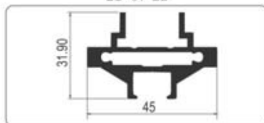
Horizontal Profile for 10mm Glass Finish : Black Matt
