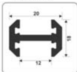
Profile for 12mm Glass (20mm) Finish : Black Matt
