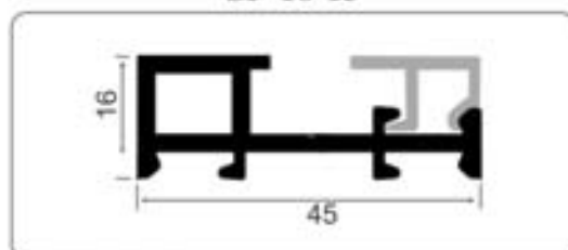
SP-16-15
