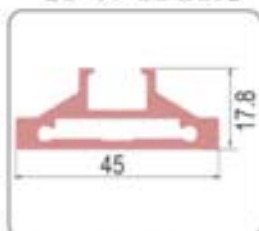
Vertical Profile Finish : Brush Rose Gold
