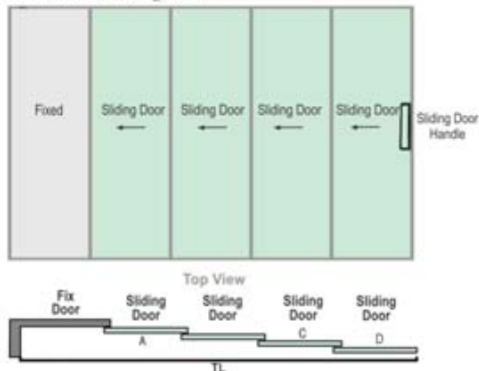
Telescopic Sliding Door Hardware for 1 Fix + 4 Sliding Door
