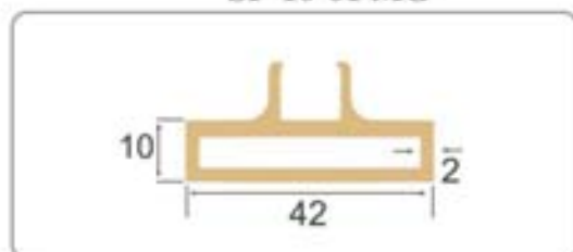
Vertical Profile For 10mm Glass (10mmx42mm) Finish : Metallic Gold Available in : 10ft and 16ft
