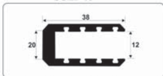
Edge Profile for 12mm Glass (38mm) Finish : Black Matt
