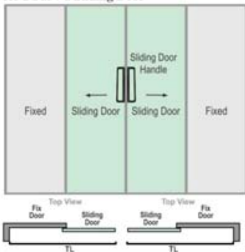
Synchronized Sliding Door Hardware for 2 Fix + 2 Sliding Door
