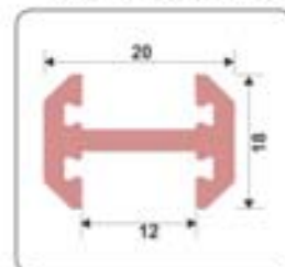
Profile for 12mm Glass (20mm) Finish : Brush Rose Gold
