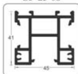
Slim Profile (25mmx45mm) Finish : Black Matt Available in : 10ft.
