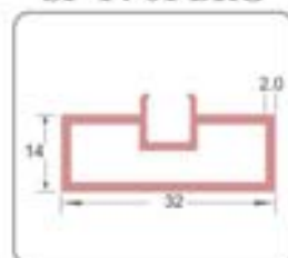
Vertical Profile For 8mm Glass (14mmx32mm) Finish : Brush Rose Gold Available in : 10ft and 16ft
