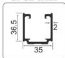
Sliding Top Track For Slim Profile Finish : Black Matt, Available in : 2, 3, 4, 6mtr.
