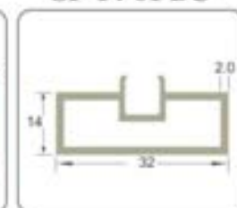
Vertical Profile For 8mm Glass (14mmx32mm) Finish : Brush Champagne Available in : 10ft and 16ft
